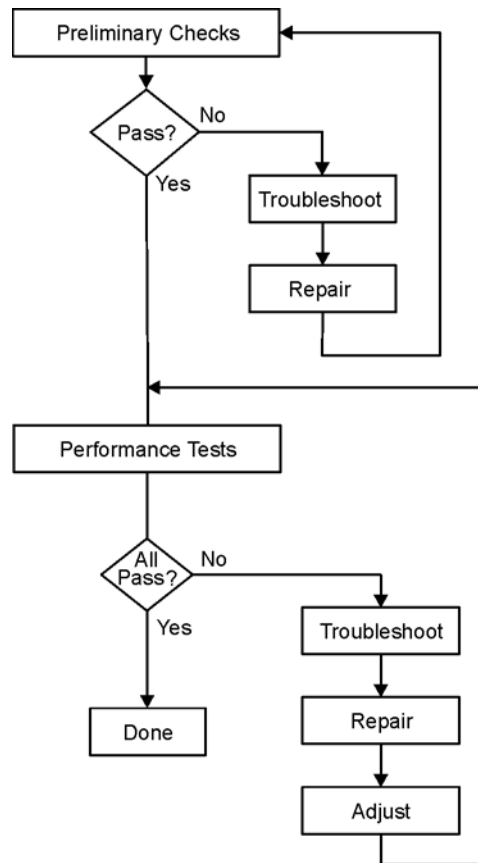
Figure 2-1 ANSI/NCSL Z524.3-2006 and ISO/IEC 17025 Verification Flowchart
