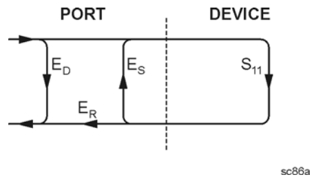
Figure 1-1 Flowgraph of 1-Port Error Terms for Port 1
